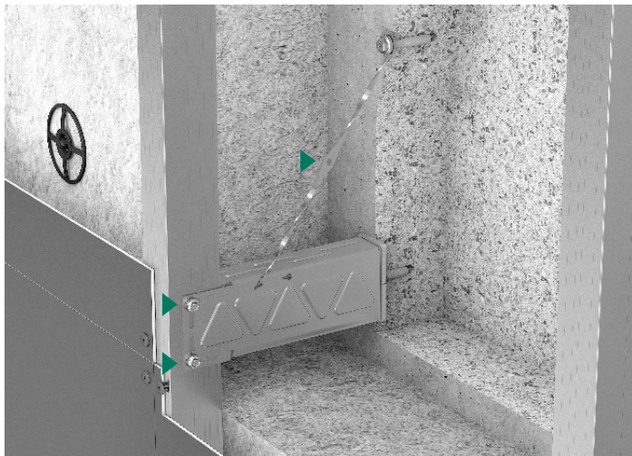
Fixed point: Fixing in a circular hole, completed by a hinge for reliable transfer of own weight.
